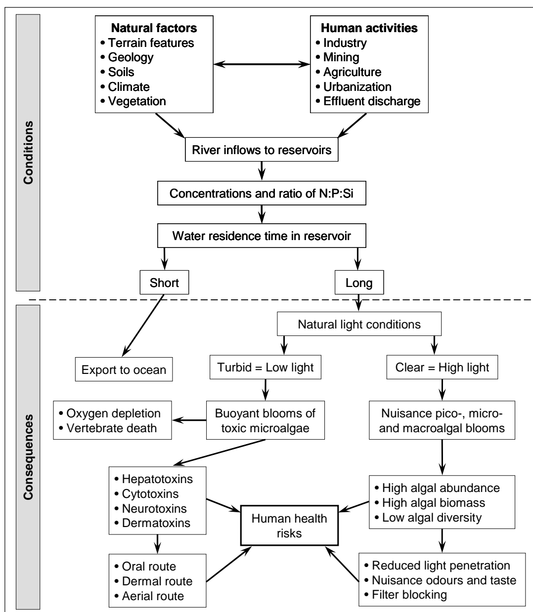
Figure 2. Overview of the sequence of interacting factors and the potential consequences of nutrient enrichment of freshwater in a man-made impoundment.
